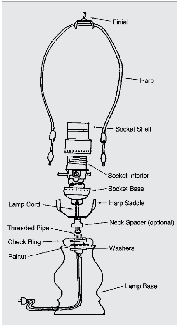
Sample illustration of an assembled lamp kit.
